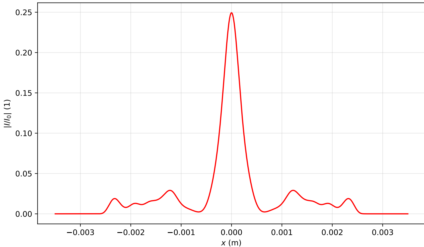
Intensity profile I(x, y = 0, z = 3.821)/I_0 , P_{in}=9.0P_{cr} , artificial time
